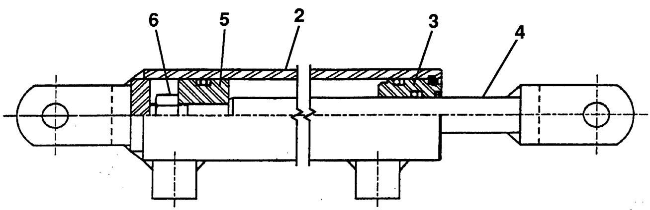
Steer Cylinder Internal Components (Type 1 Cylinder shown)
